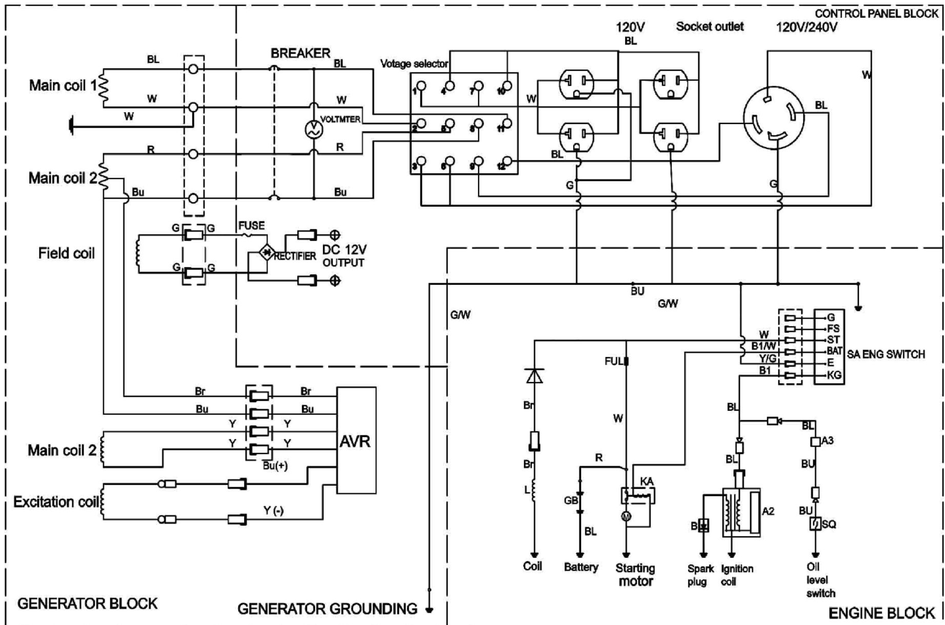
LF8500iE, LF8500iE-CA, LF8500iEPL, & LF8500iEPL-CA Wiring Diagram
