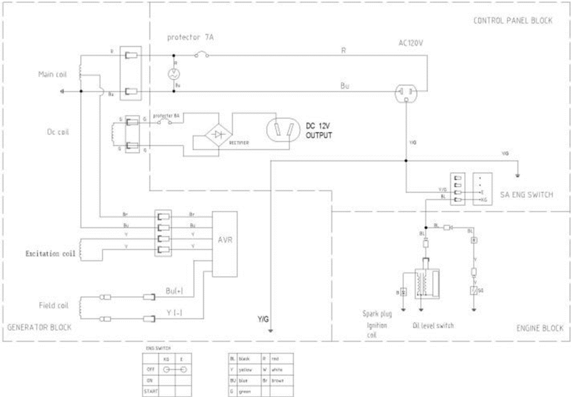
WIRING DIAGRAM
